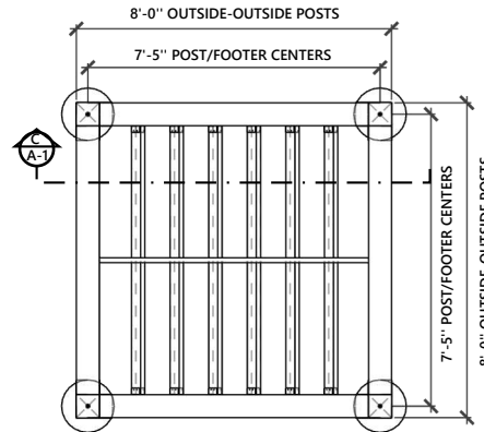
POST/FOOTER LAYOUT/ TOP VIEW
