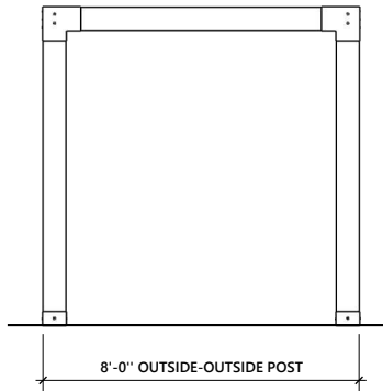
LEFT AND RIGHT ELEVATION
