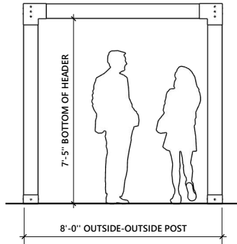
FRONT AND REAR ELEVATION
