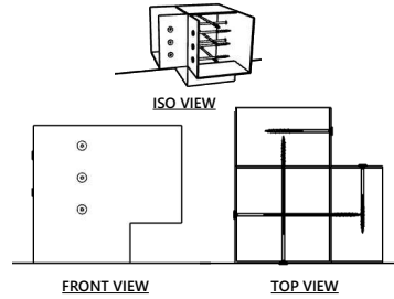
POST-BEAM CORNER BRACKET
