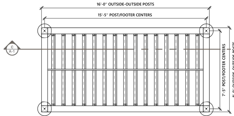
POST/FOOTER LAYOUT/ TOP VIEW
