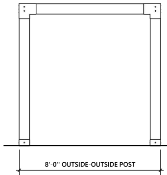
LEFT AND RIGHT ELEVATION
