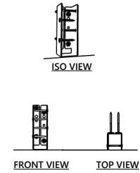
RAFTER-BEAM BRACKET
