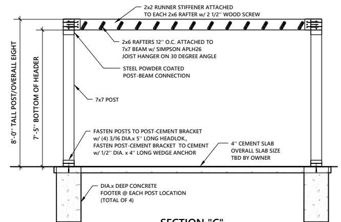
SECTION "C"
