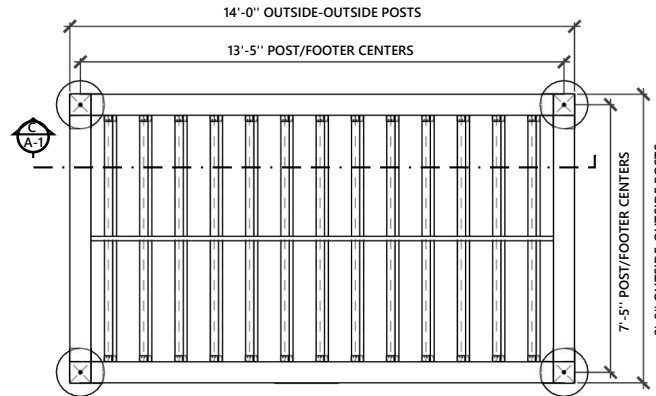
POST/FOOTER LAYOUT/ TOP VIEW
