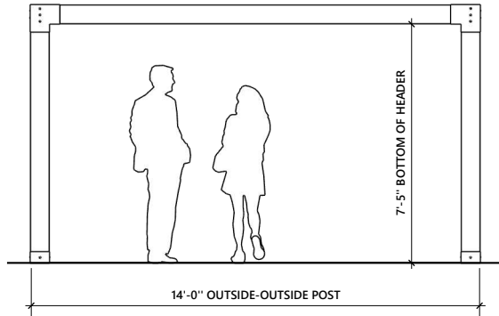
FRONT AND REAR ELEVATION
