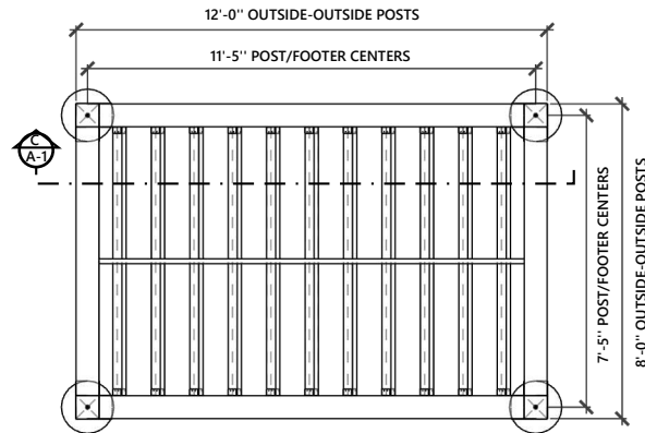
POST/FOOTER LAYOUT/ TOP VIEW
