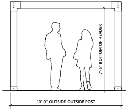
FRONT AND REAR ELEVATION
