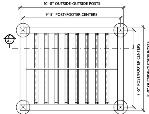
POST/FOOTER LAYOUT/ TOP VIEW
