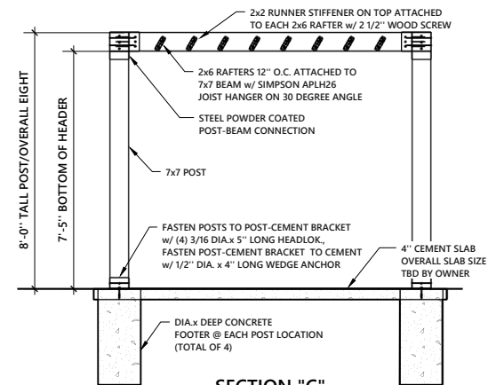
SECTION "C"
