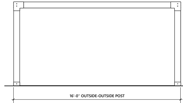
LEFT AND RIGHT ELEVATION
