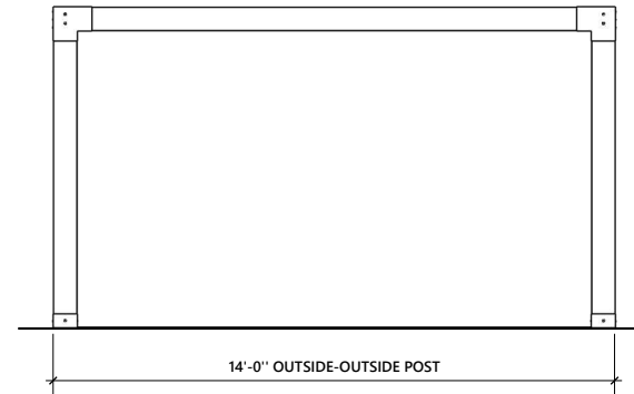
LEFT AND RIGHT ELEVATION
