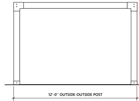
LEFT AND RIGHT ELEVATION
