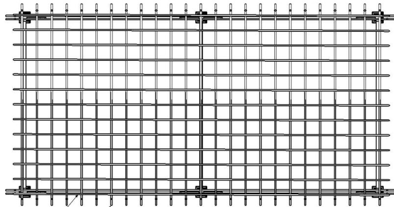
2x8 HEADER 2x6 RUNNER TOP VIEW SCALE: 3/16" = 1'-0"
