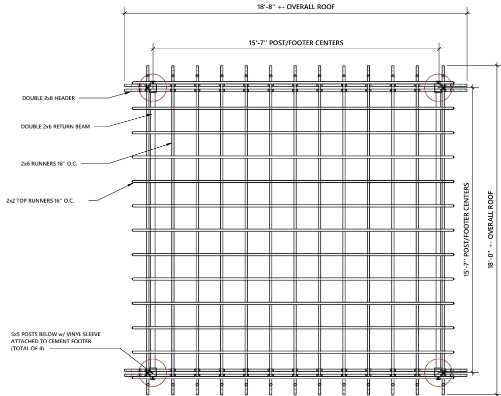
POST/FOOTER PLAN/ TOP VIEW
