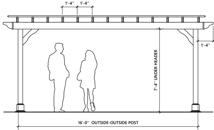
FRONT AND REAR VIEW
