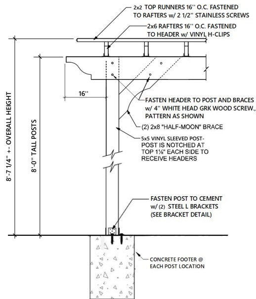
HEADER-POST CONNECTION
