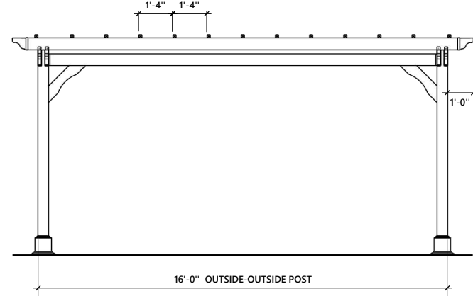
LEFT AND RIGHT VIEW
