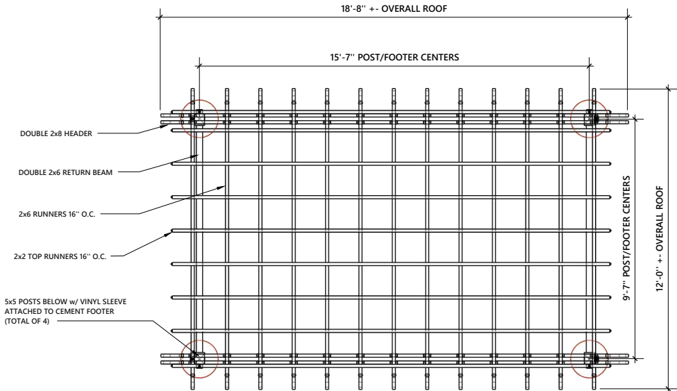
POST/FOOTER PLAN/ TOP VIEW
