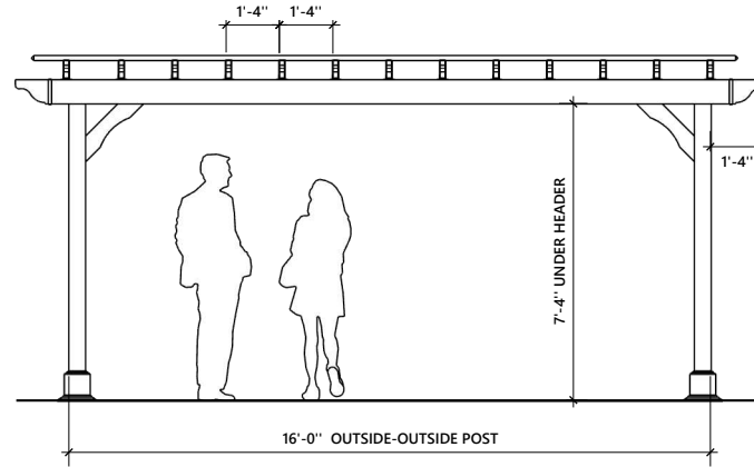
FRONT AND REAR VIEW
