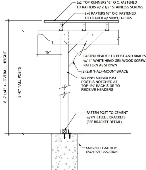
HEADER-POST CONNECTION
