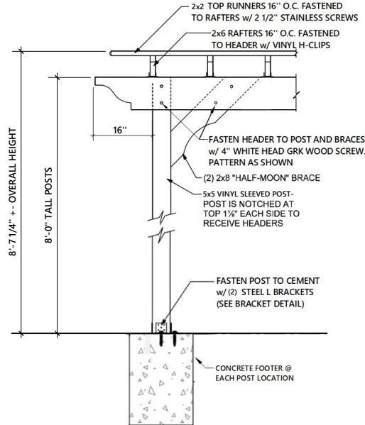
HEADER-POST CONNECTION
