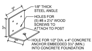
STEEL L-BRACKET DETAIL NO SCALE
