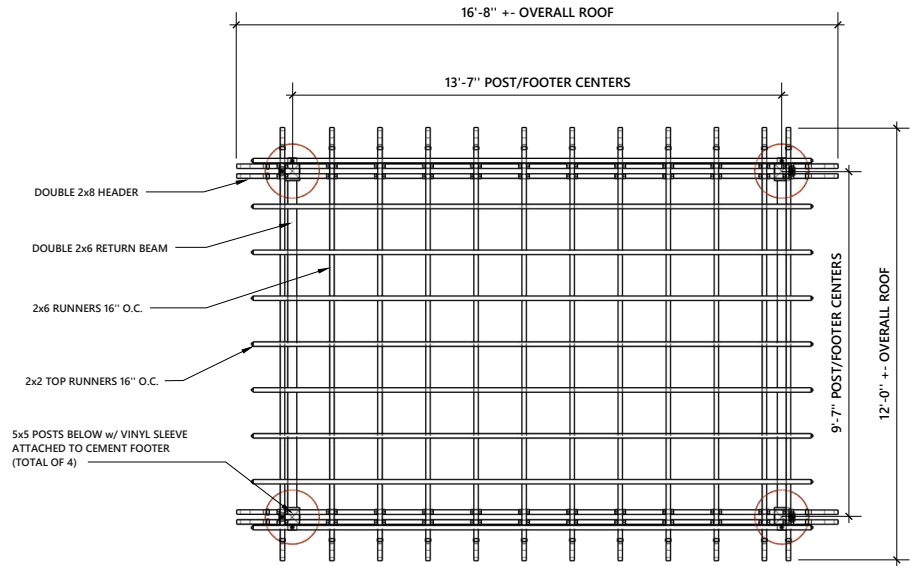
POST/FOOTER PLAN/ TOP VIEW
