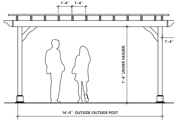
FRONT AND REAR VIEW
