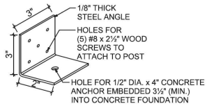
STEEL L-BRACKET DETAIL NO SCALE
