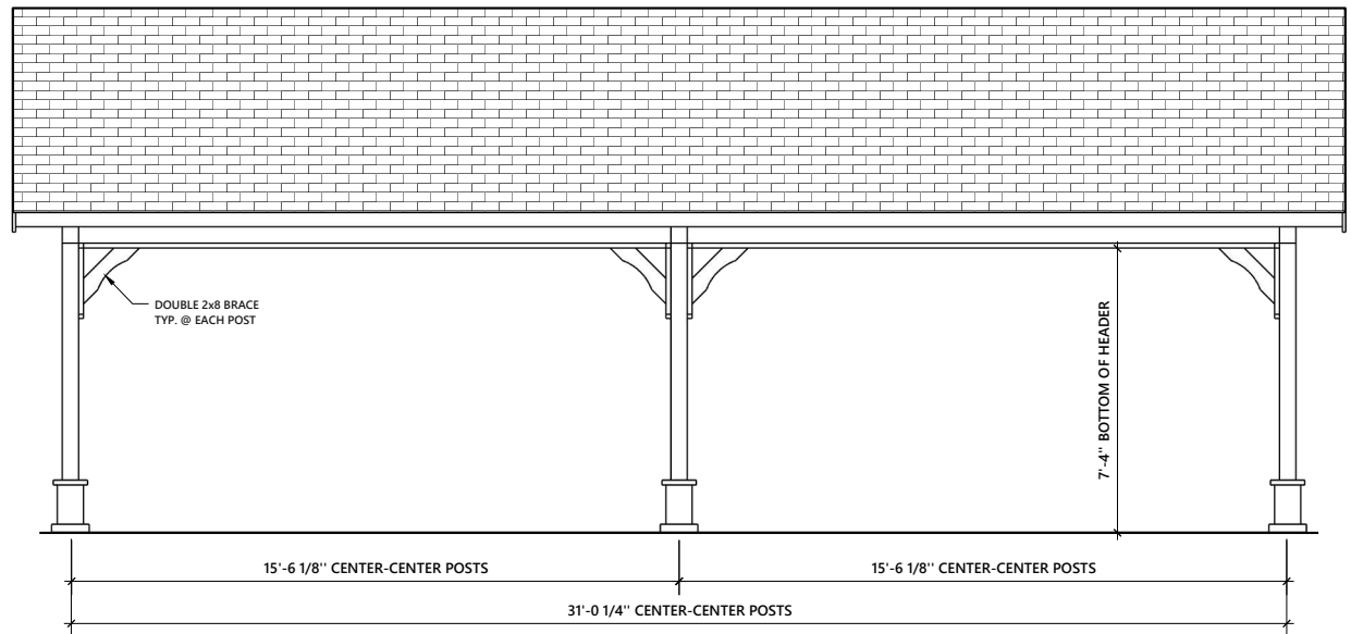
FRONT AND REAR ELEVATION
