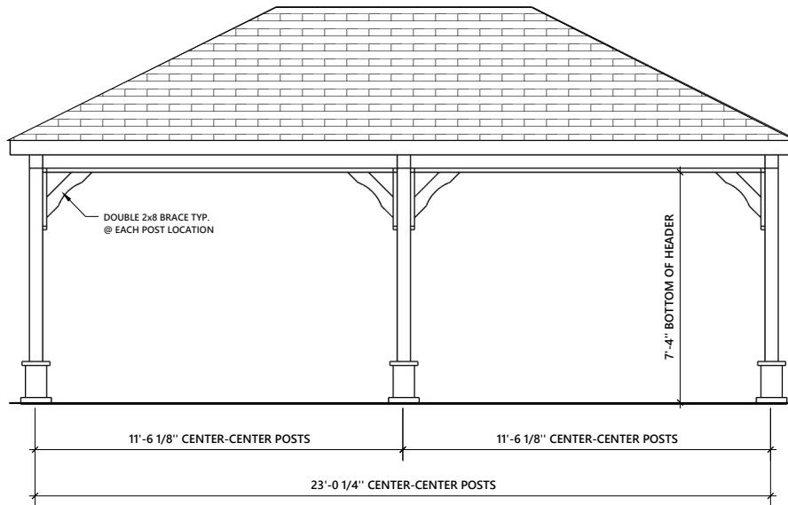
FRONT AND REAR ELEVATION
