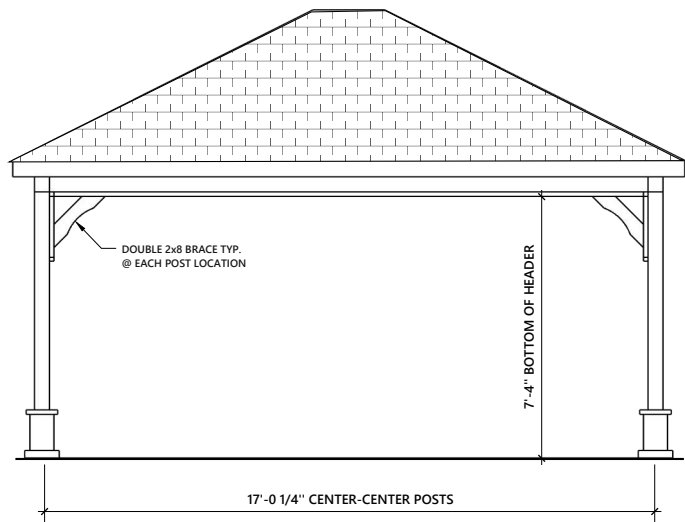
FRONT AND REAR ELEVATION
