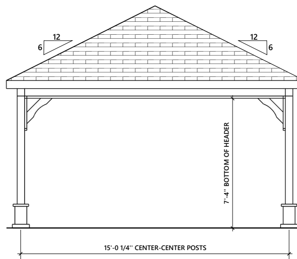
LEFT AND RIGHT ELEVATION
