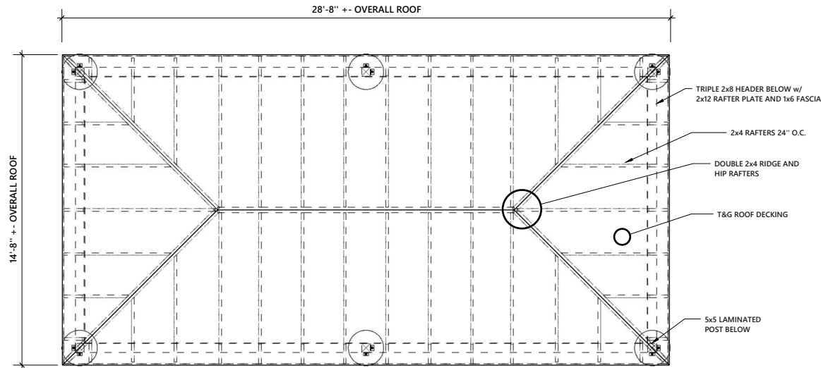
ROOF FRAMING PLAN
