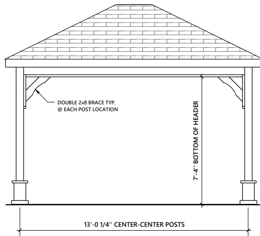
FRONT AND REAR ELEVATION
