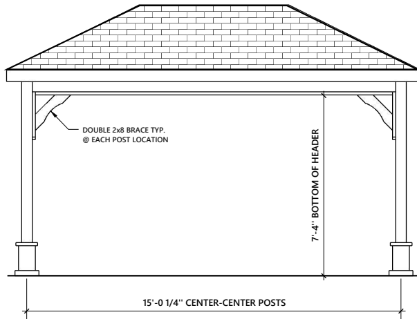
FRONT AND REAR ELEVATION
