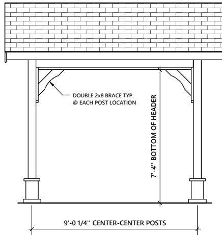
FRONT AND REAR ELEVATION
