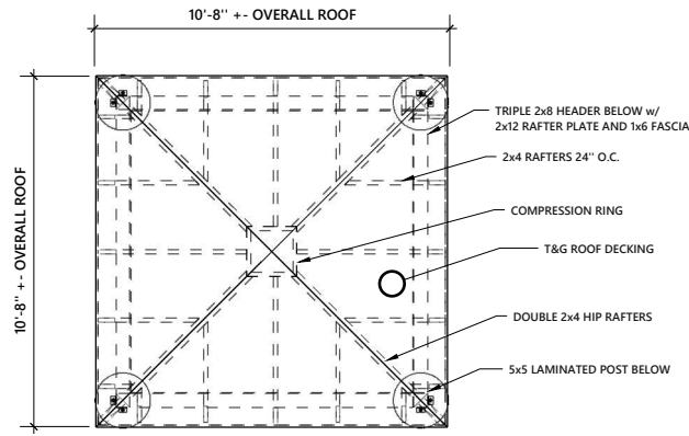
ROOF FRAMING PLAN
