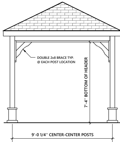
FRONT AND REAR ELEVATION
