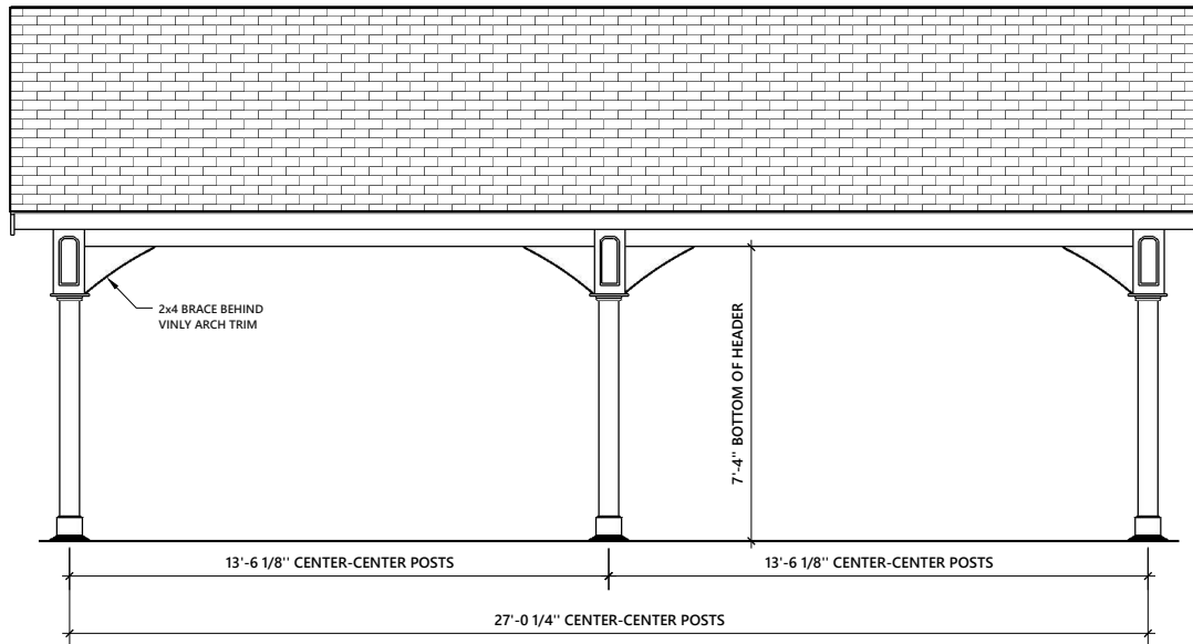
FRONT AND REAR ELEVATION
