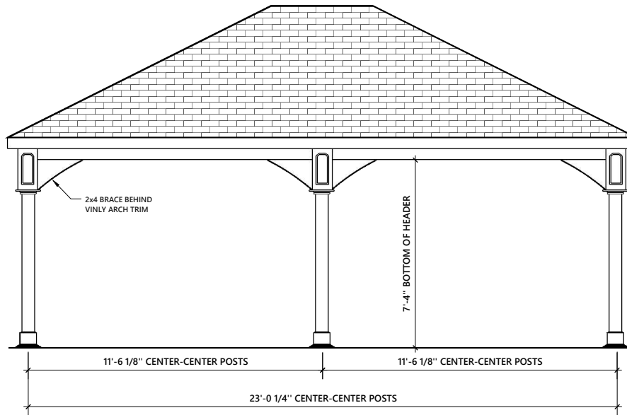
FRONT AND REAR ELEVATION
