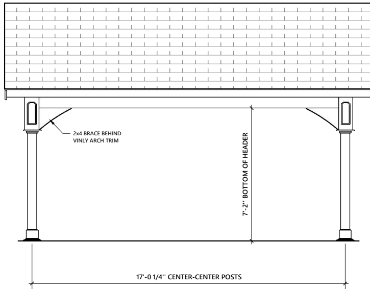
FRONT AND REAR ELEVATION
