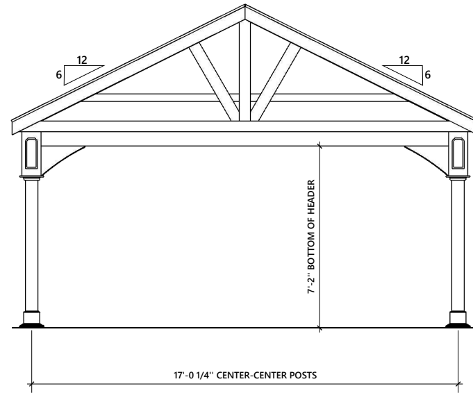
LEFT AND RIGHT ELEVATION
