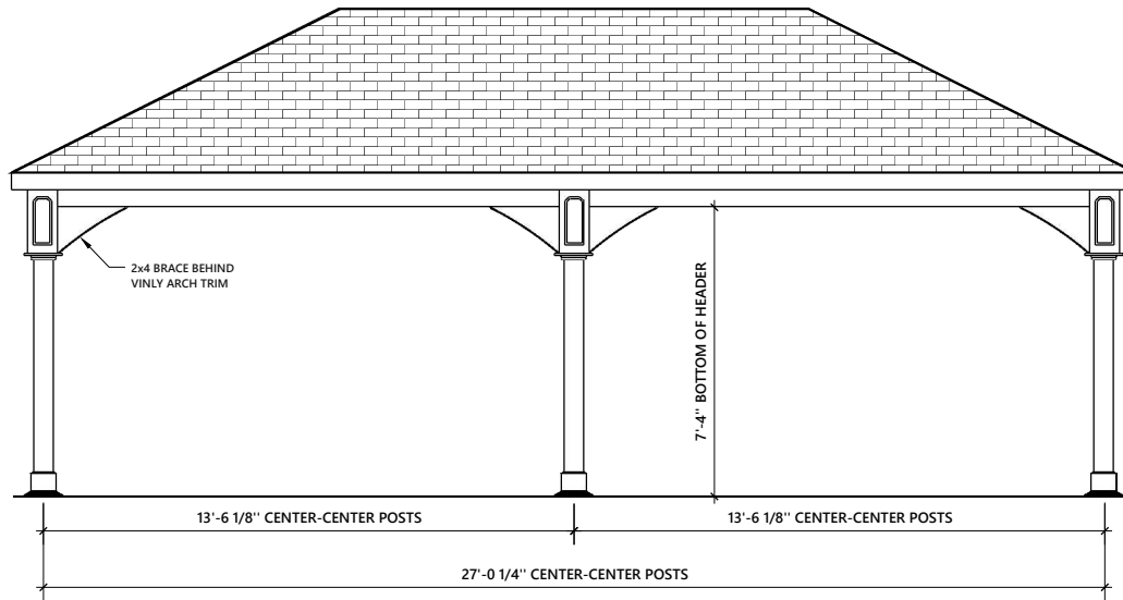
FRONT AND REAR ELEVATION
