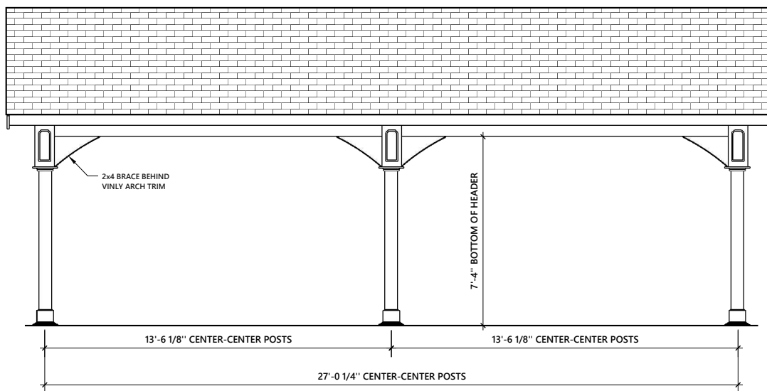
FRONT AND REAR ELEVATION
