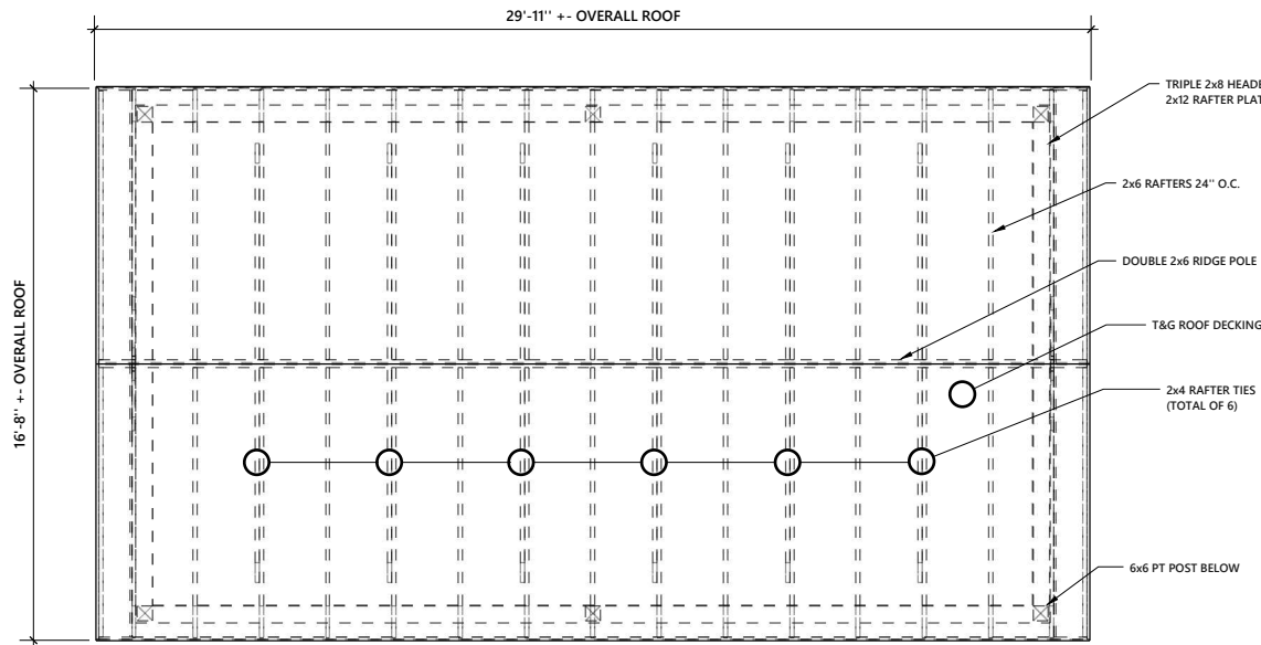
ROOF FRAMING PLAN
