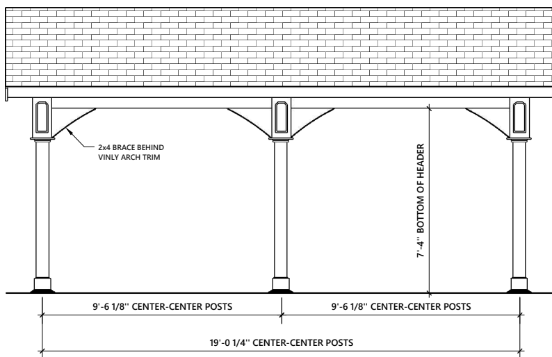
FRONT AND REAR ELEVATION
