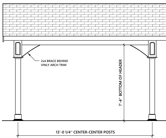
FRONT AND REAR ELEVATION
