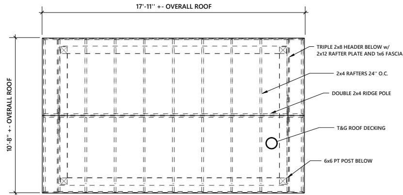
ROOF FRAMING PLAN
