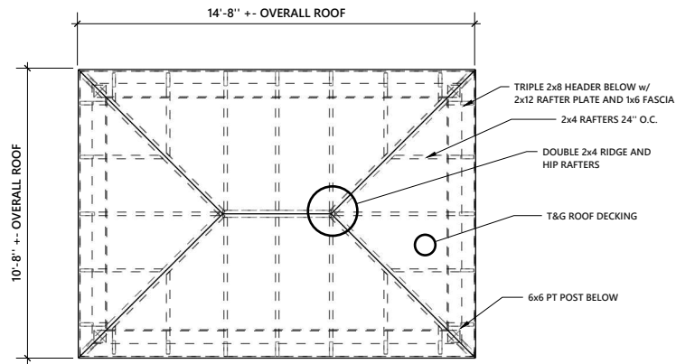
ROOF FRAMING PLAN
