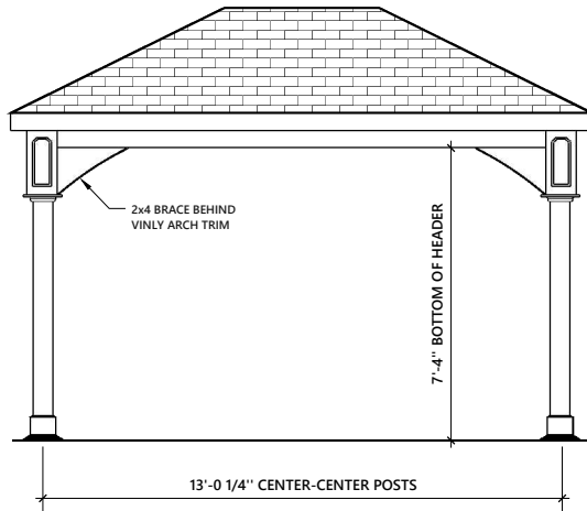
FRONT AND REAR ELEVATION
