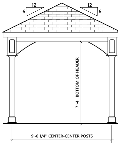
LEFT AND RIGHT ELEVATION
