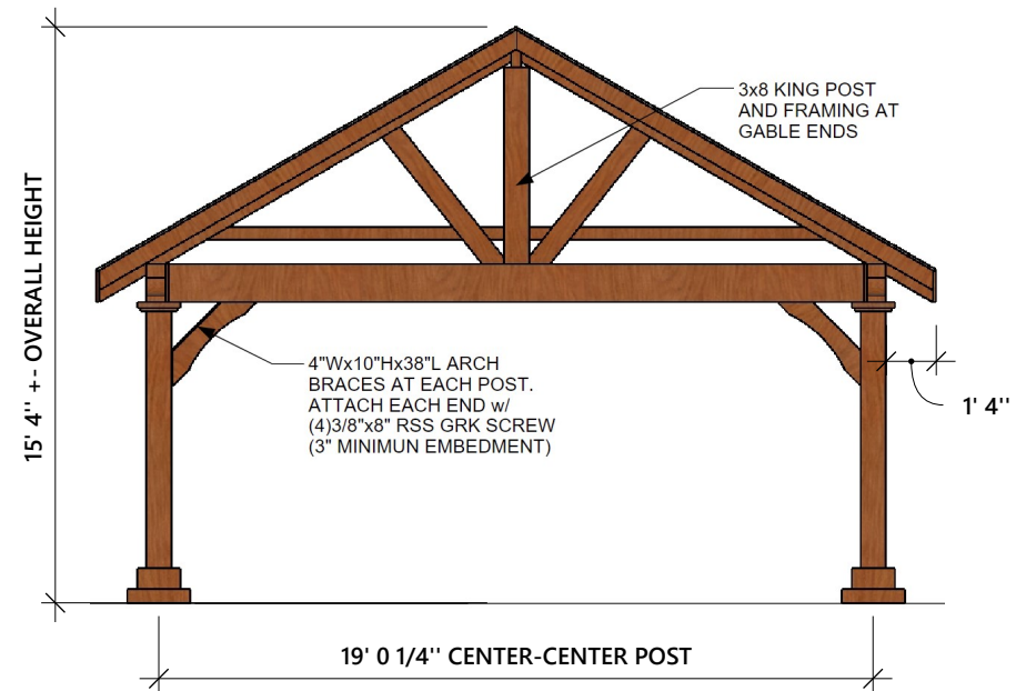
LEFT AND RIGHT ELEVATION
