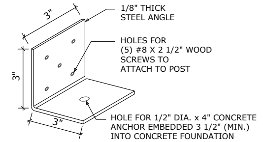
POST L BRACKET DETAIL NO SCALE
