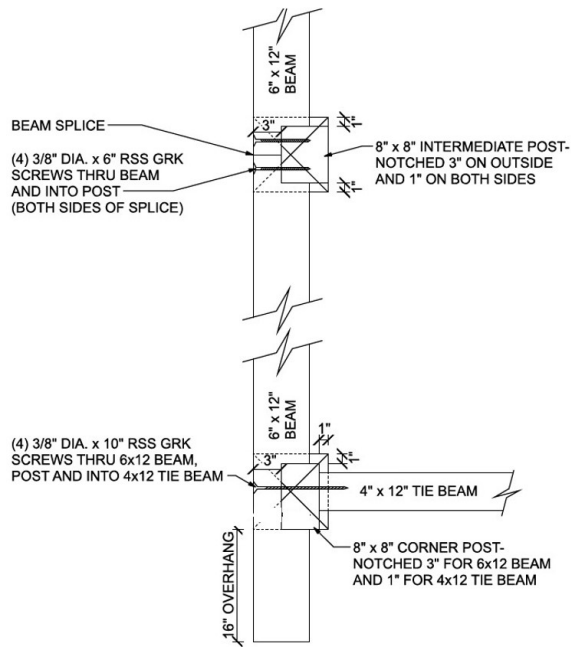
BEAM / POST / TIE BEAM CONNECTION DETAIL
