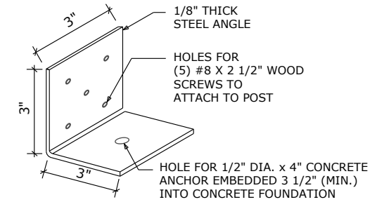
POST L BRACKET DETAIL NO SCALE
