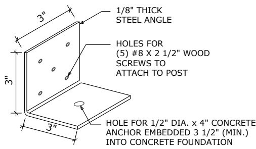
POST L BRACKET DETAIL NO SCALE
