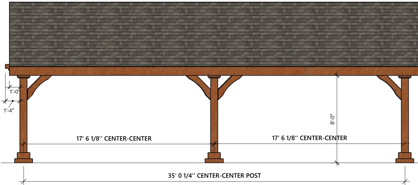
FRONT AND REAR ELEVATION
