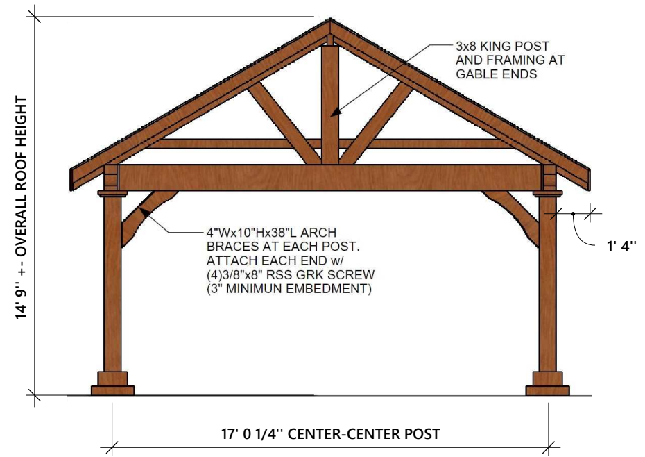
LEFT AND RIGHT ELEVATION
