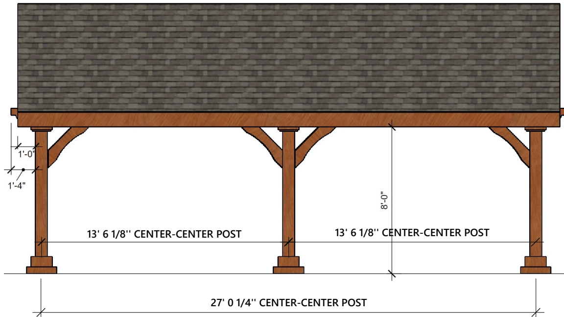
FRONT AND REAR ELEVATION
