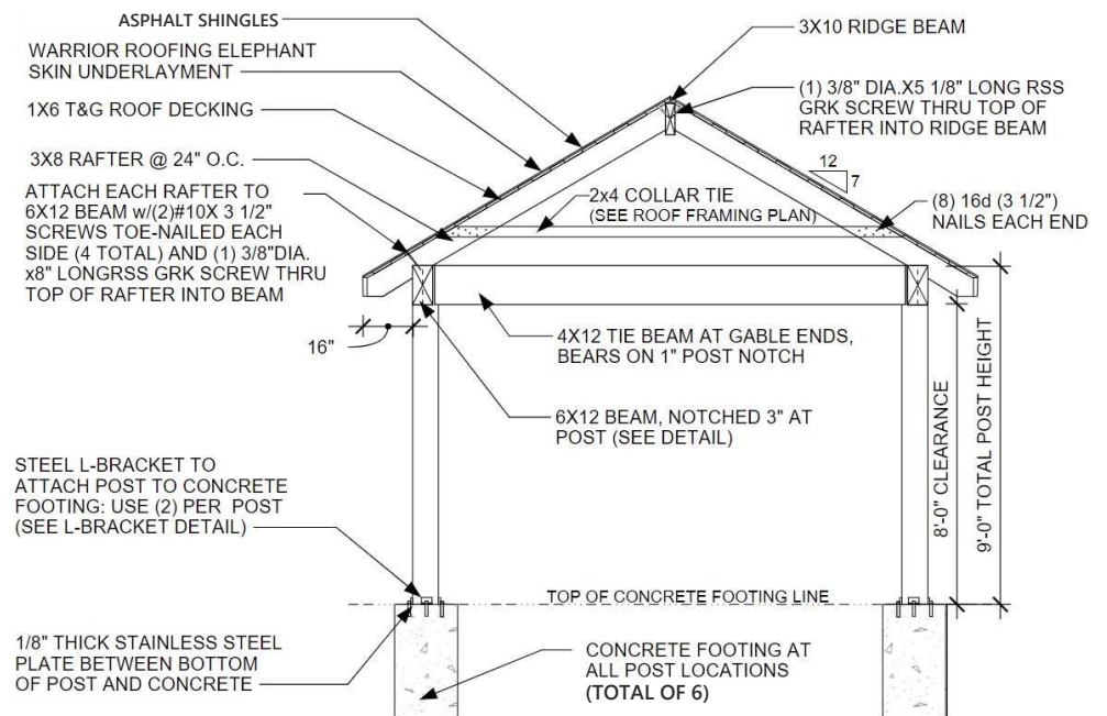
CROSS SECTION
