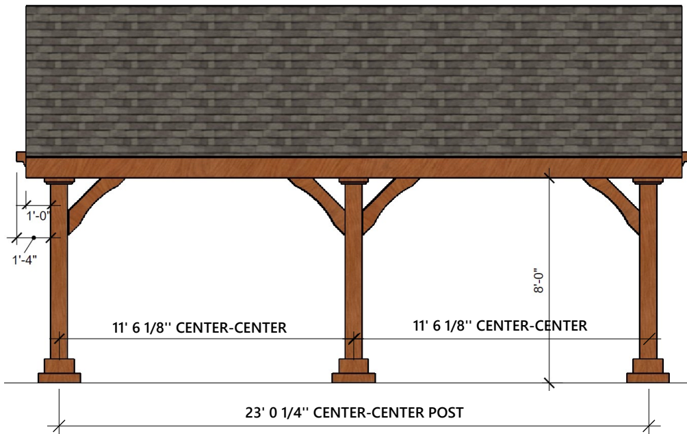
FRONT AND REAR ELEVATION
