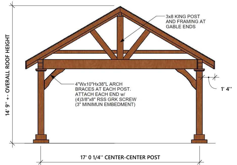
LEFT AND RIGHT ELEVATION
