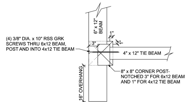
BEAM / POST / TIE BEAM CONNECTION DETAIL
