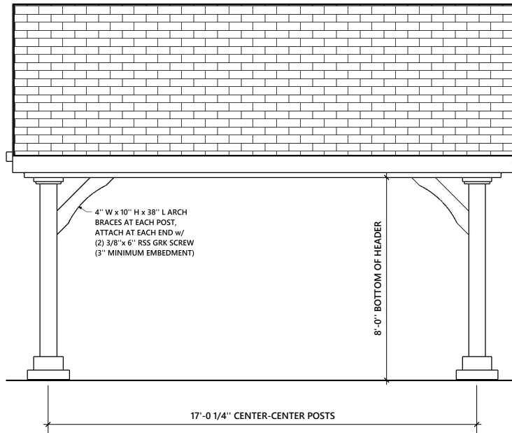
FRONT AND REAR ELEVATION
