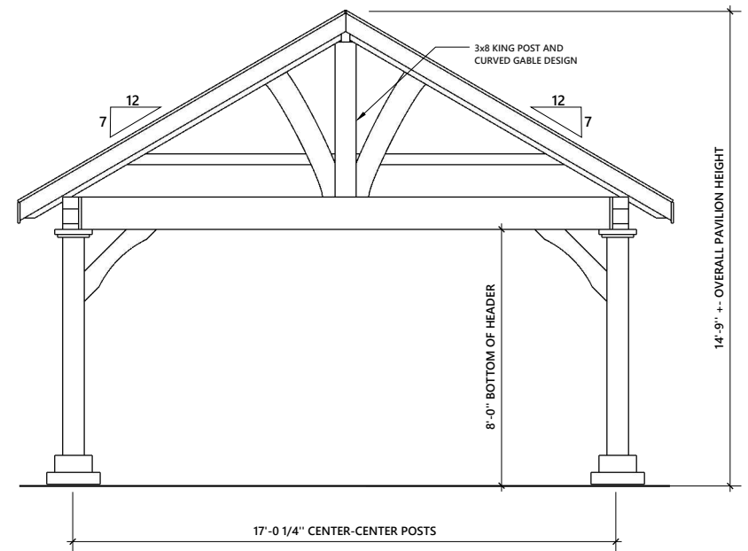
LEFT AND RIGHT ELEVATION
