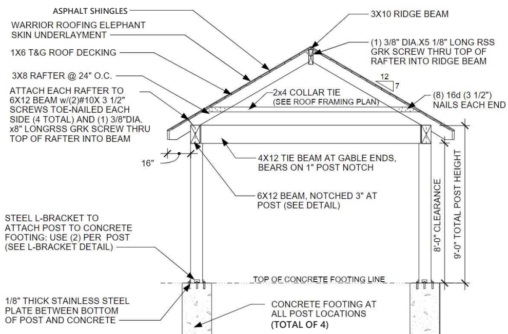
CROSS SECTION
