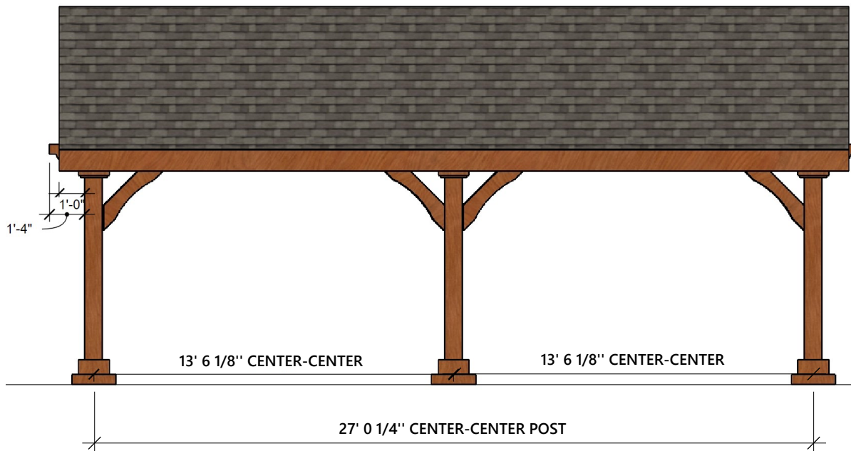
FRONT AND REAR ELEVATION
