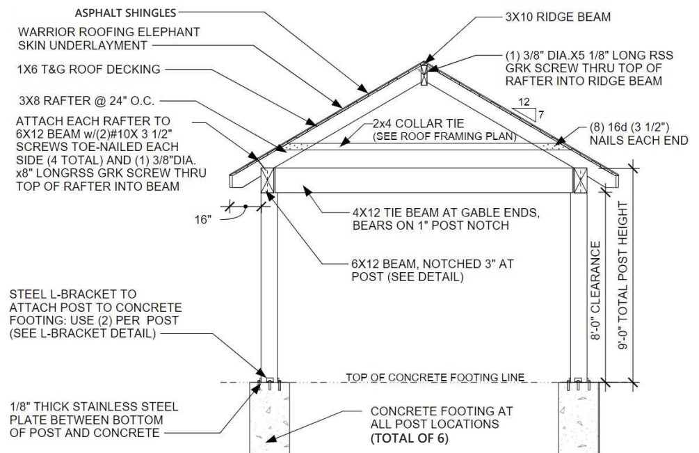
CROSS SECTION
