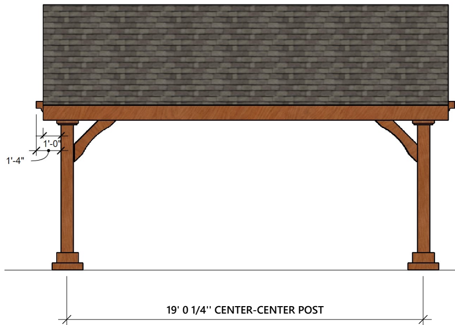
FRONT AND REAR ELEVATION
