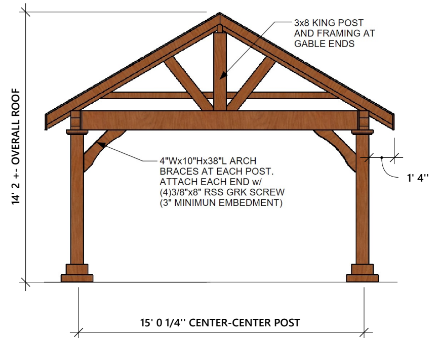
LEFT AND RIGHT ELEVATION
