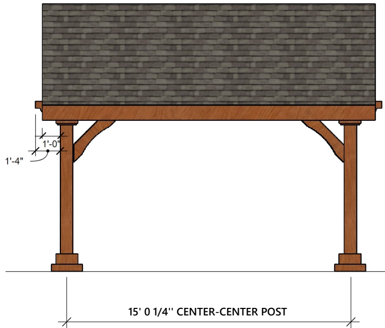
FRONT AND REAR ELEVATION
