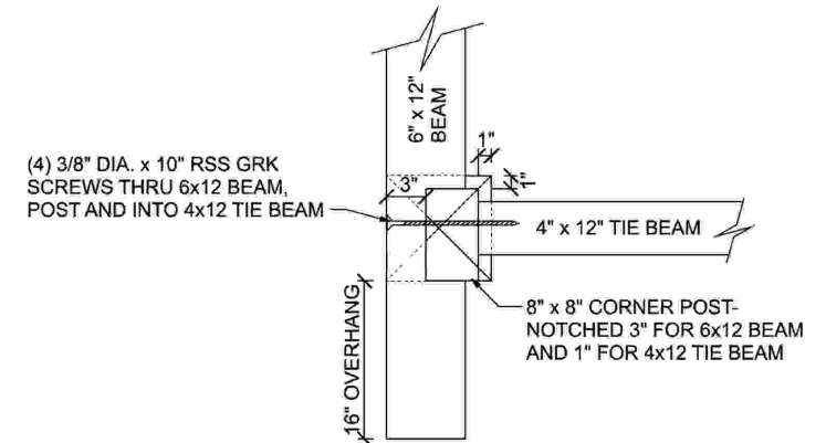
BEAM / POST / TIE BEAM CONNECTION DETAIL
