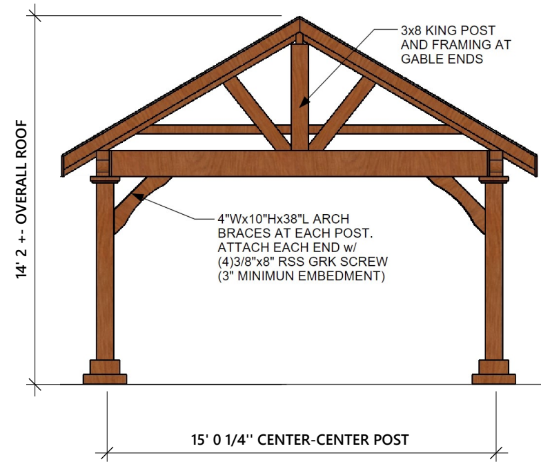
LEFT AND RIGHT ELEVATION
