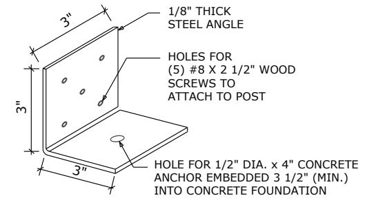
POST L BRACKET DETAIL NO SCALE
