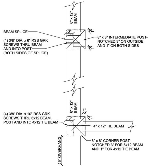
BEAM / POST / TIE BEAM CONNECTION DETAIL
