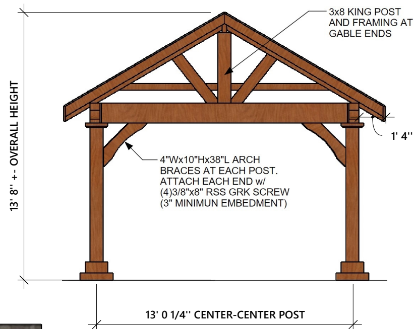
LEFT AND RIGHT ELEVATION
