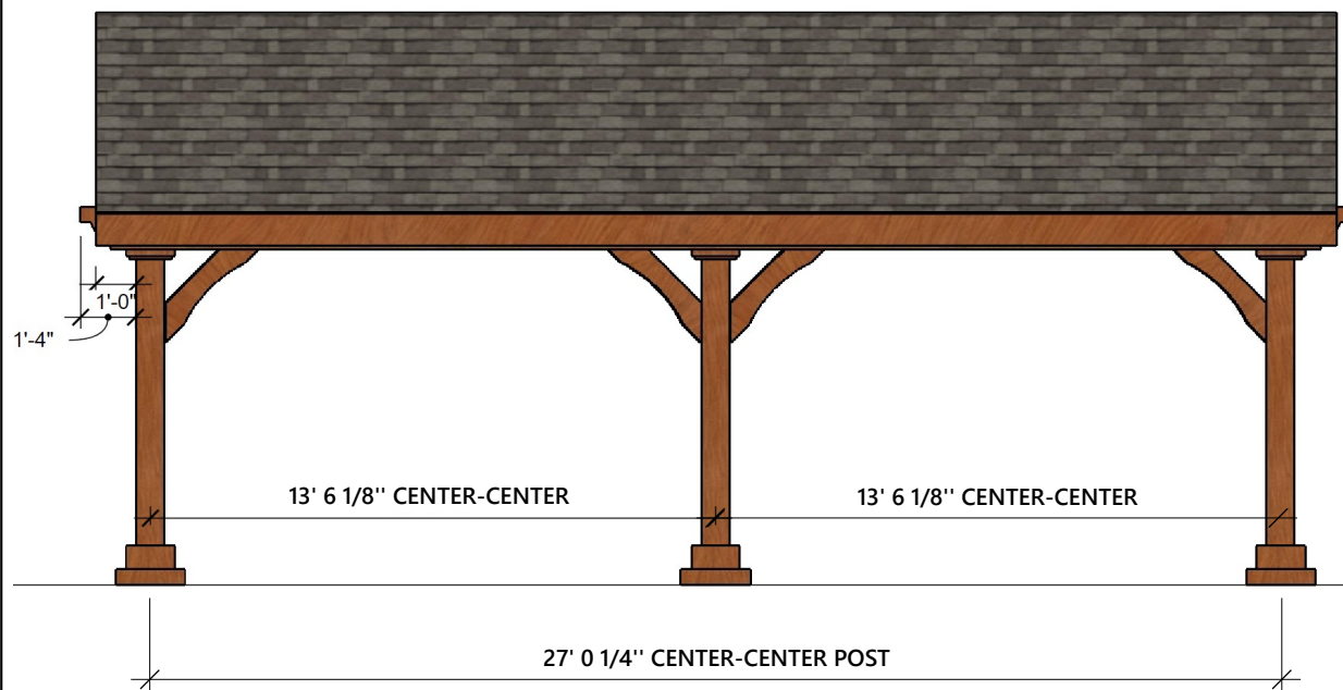
FRONT AND REAR ELEVATION
