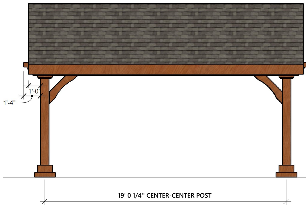
FRONT AND REAR ELEVATION
