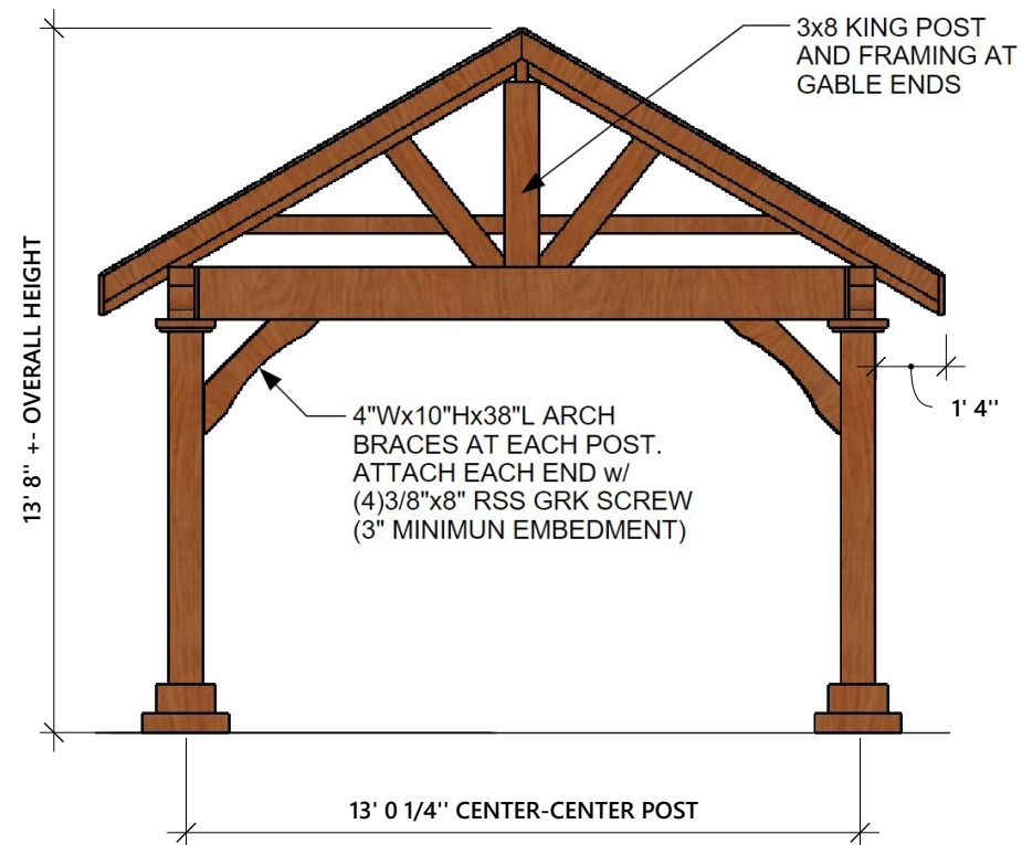
LEFT AND RIGHT ELEVATION
