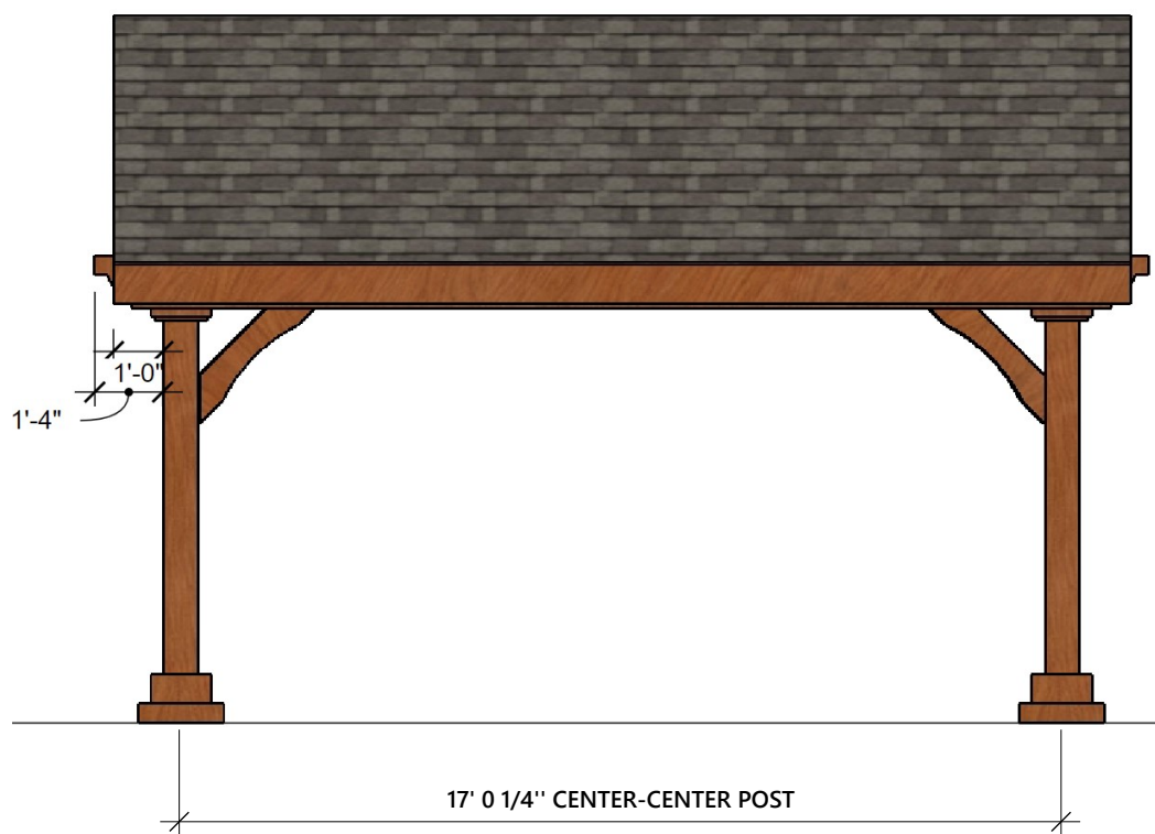
FRONT AND REAR ELEVATION
