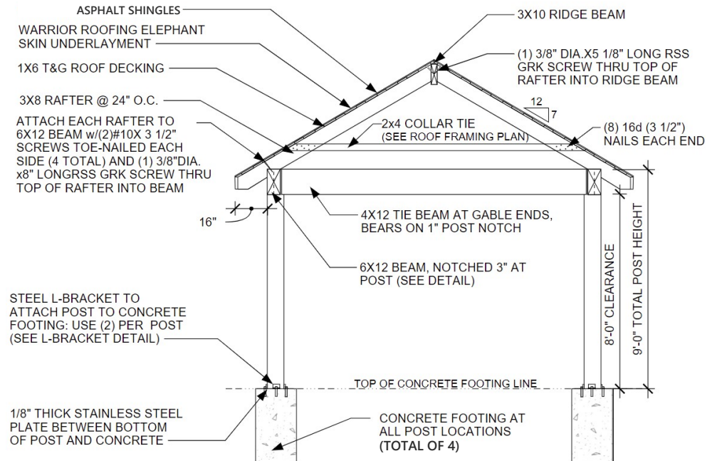
CROSS SECTION
