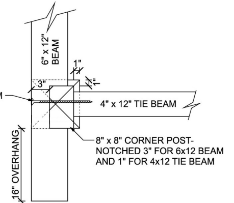
BEAM / POST / TIE BEAM CONNECTION DETAIL
