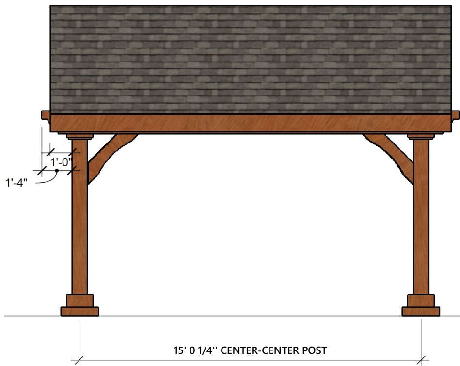
FRONT AND REAR ELEVATION
