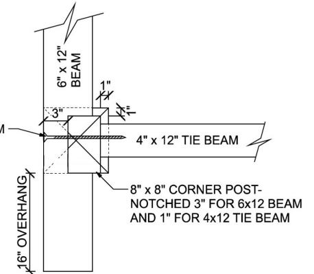
BEAM / POST / TIE BEAM CONNECTION DETAIL
