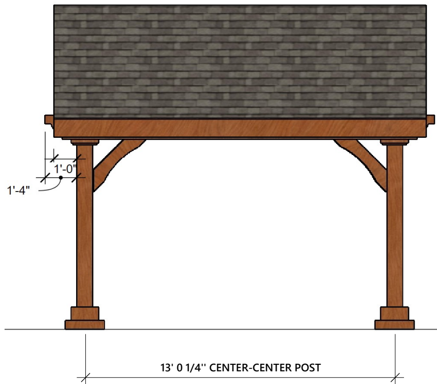
FRONT AND REAR ELEVATION
