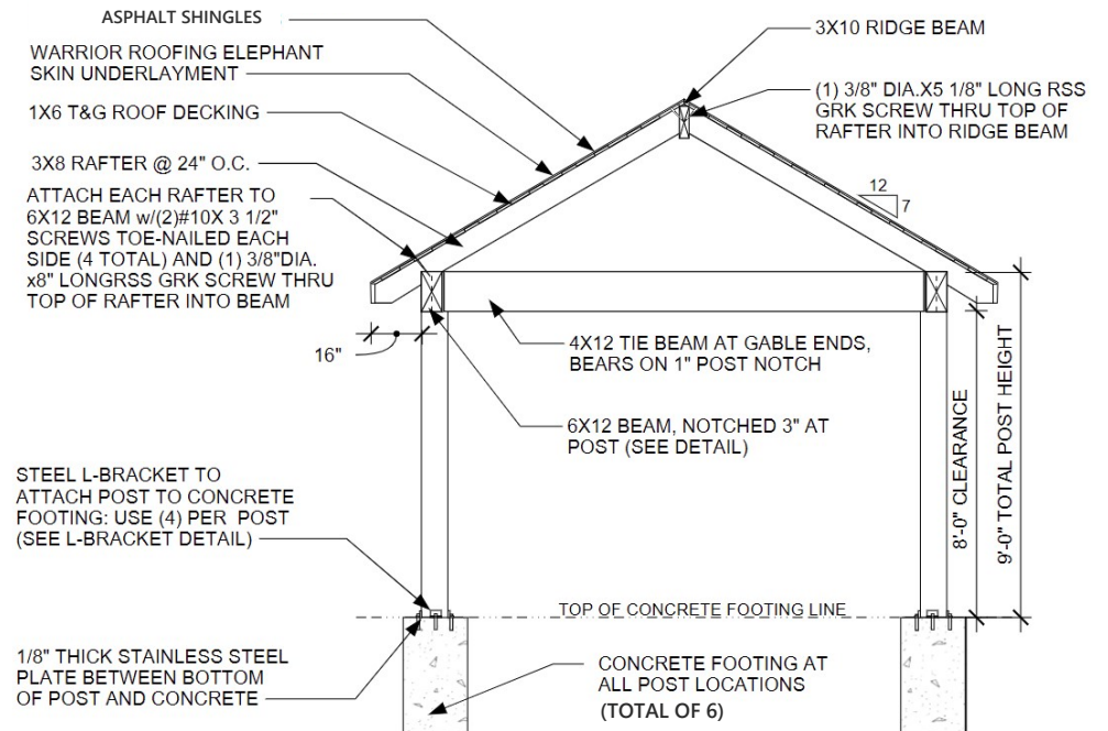
CROSS SECTION
