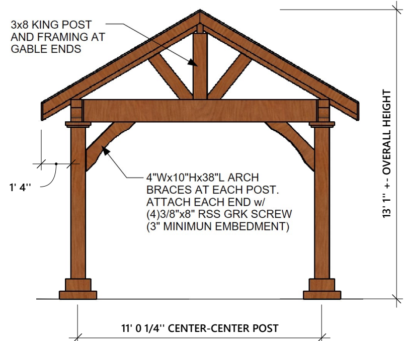
LEFT AND RIGHT ELEVATION
