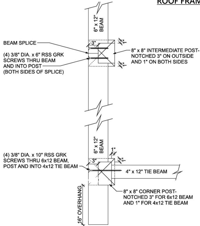
BEAM / POST / TIE BEAM CONNECTION DETAIL
