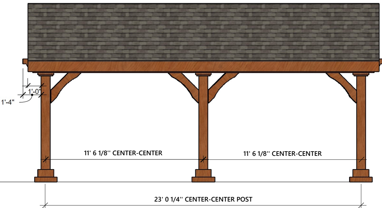
FRONT AND REAR ELEVATION
