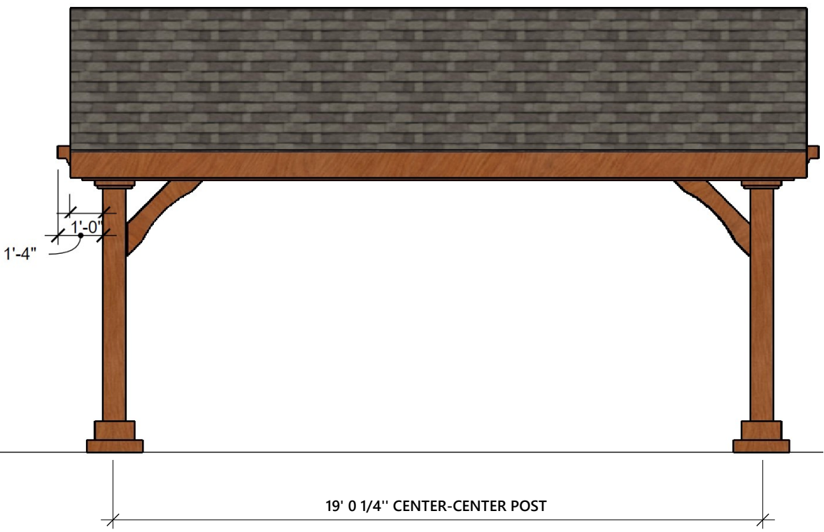
FRONT AND REAR ELEVATION
