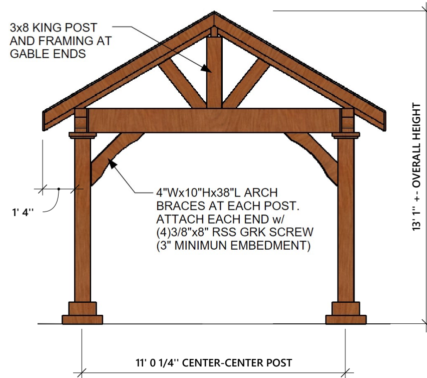
LEFT AND RIGHT ELEVATION
