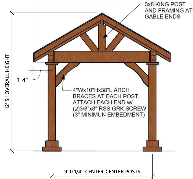
LEFT AND RIGHT ELEVATION
