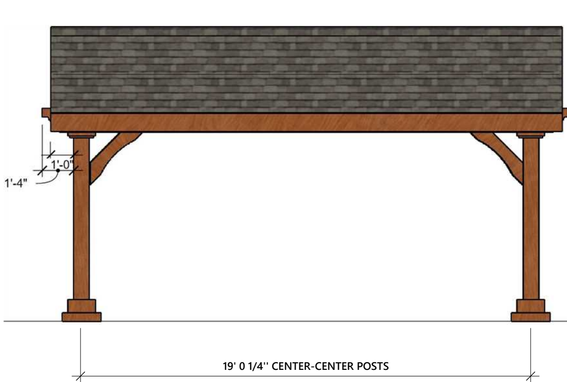
FRONT AND REAR ELEVATION
